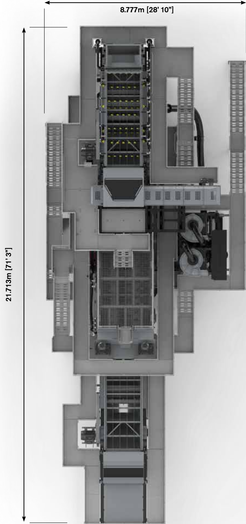
AGGWASH 300 WORKING DIMENSIONS PLAN VIEW
